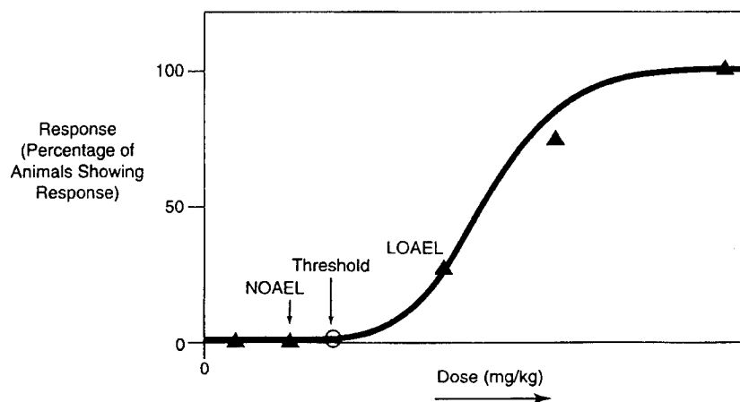
Fig 3. Depiction of a hypothetical dose-response curve. Data points are represented by triangles. The NOAEL is the highest dose that caused no significant effects (over background) in offspring. The lowest-observable adverse effect level is the lowest dose that caused significant effects (over background) in offspring. The threshold is the calculated lowest point on the dose-response curve at which a dose of test agent would elicit changes in offspring; doses below the threshold will not cause deleterious effects in offspring and should be considered safe. 9
