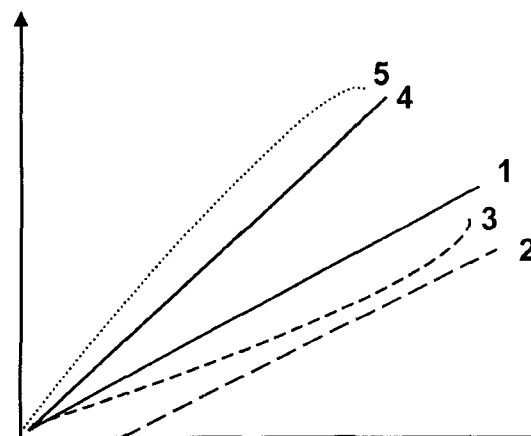
Fig 2. Examples of dose-response models used for carcinogens: 1, linear nonthreshold model; 2, linear threshold model; 3, sublinear threshold model; 4, linear nonthreshold model (steeper slope than 1 indicates greater susceptibility); and 5, supralinear nonthreshold model. Adapted from Samet and Burke. 3
