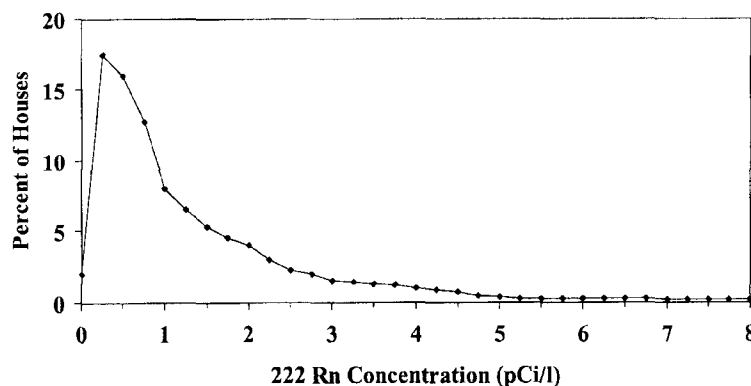
Fig 1. Distribution of radon levels in US homes. 3
