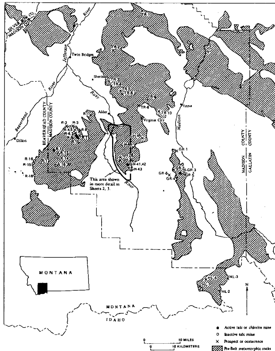
Figure 3—Talc and chlorite occurrences in southwestern Montana.
