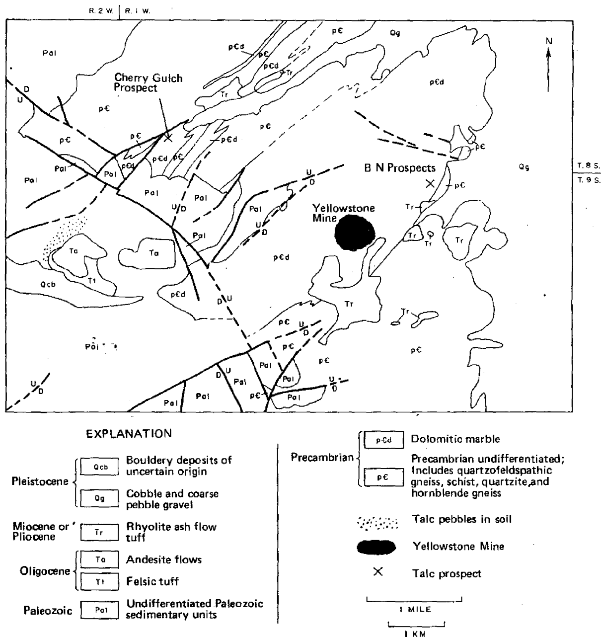
Figure 20—Generalized geologic map of the Cherry Gulch-Johnny Gulch area of the Gravelly Range. Geology from the more detailed geologic maps of the Varney and Cameron quadrangles by Hadley (1969a, 1969b).
