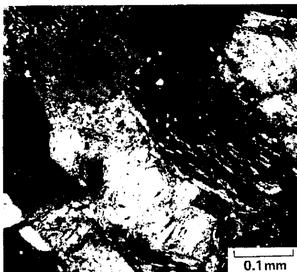
A. Slight sericitic alteration of feldspars, minor epidote and chlorite.
