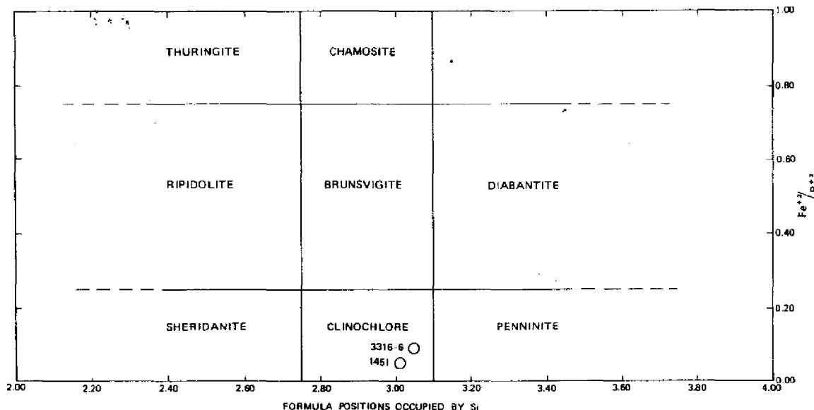
Figure 2—Plot of compositions of analyzed chlorite.
