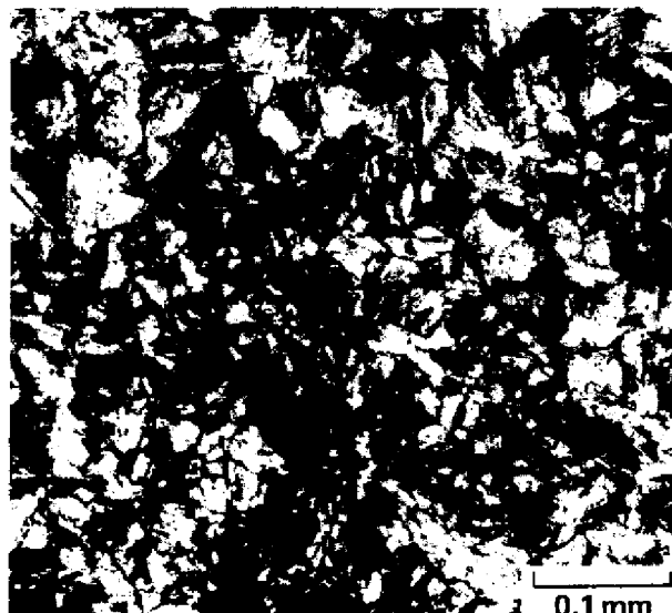
D. Specimen 3316-6 of unusually pure chlorite from the Willow Creek mine. Polars crossed.
