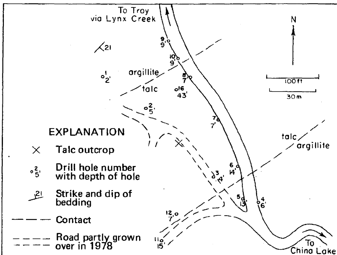
Figure 23—Lynx Creek (Mathews) talc prospect, Lincoln County (modified from Johns, 1970, p. 152).
