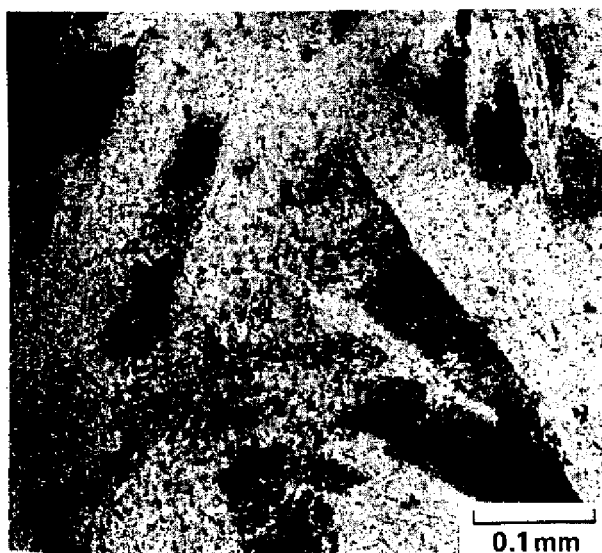
C. Specimen 1451 of chlorite that has replaced diabase dike at the Ruby claims. Relict ophitic texture shown by masses of pure chlorite that has replaced plagioclase and dark areas where chlorite-rutile mixture has replaced a pyroxene. Plane light.
