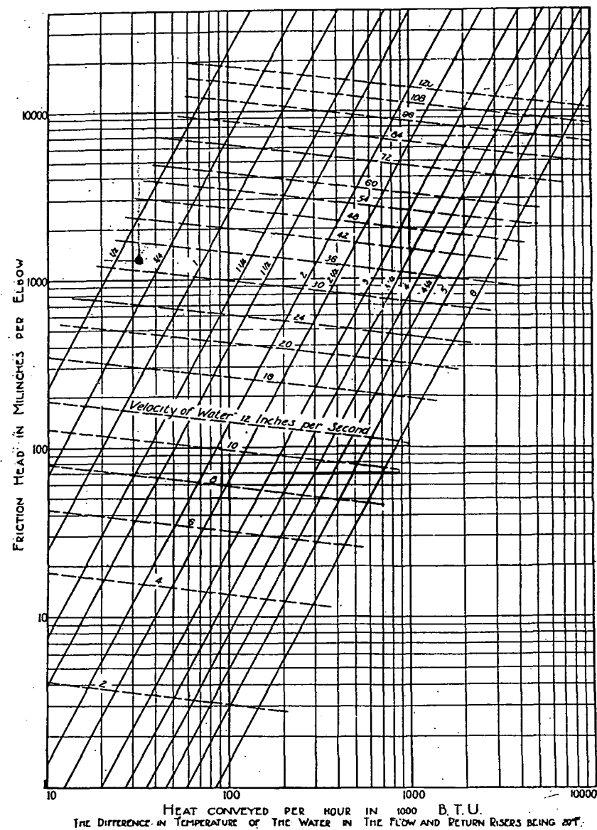
FIG. 34. CHART FOR FINDING THE FRICTION HEAD PER ELBOW
