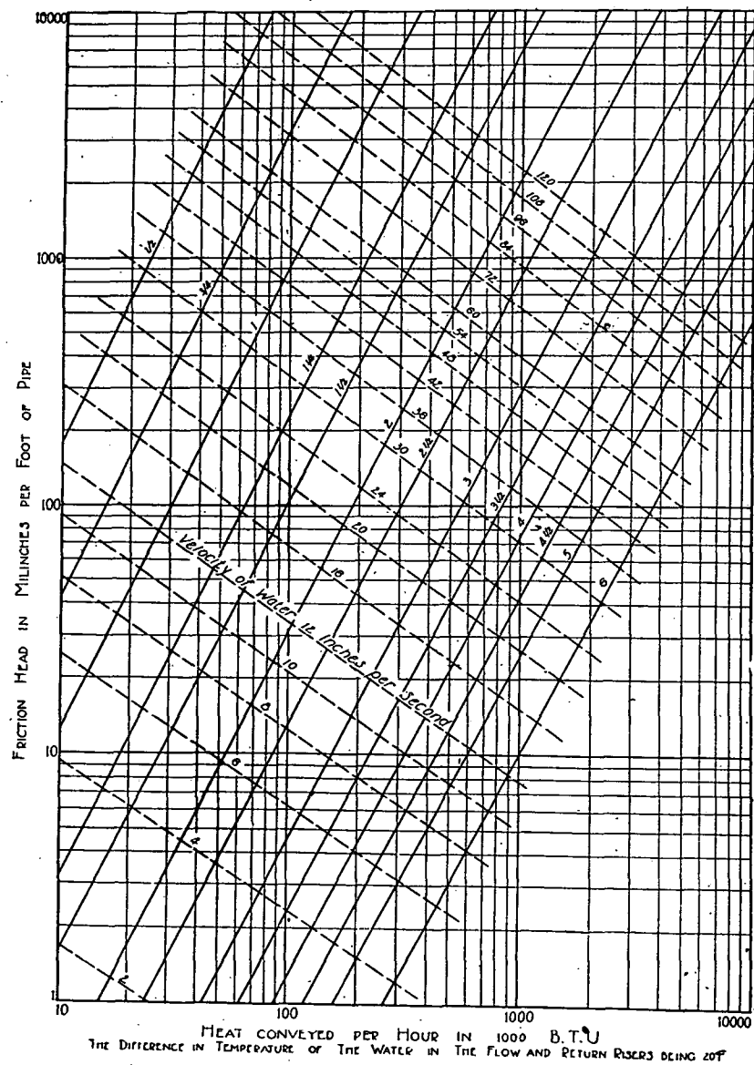
FIG. 33. CHART FOR FINDING FRICTION HEAD PER FOOT OF PIPE
