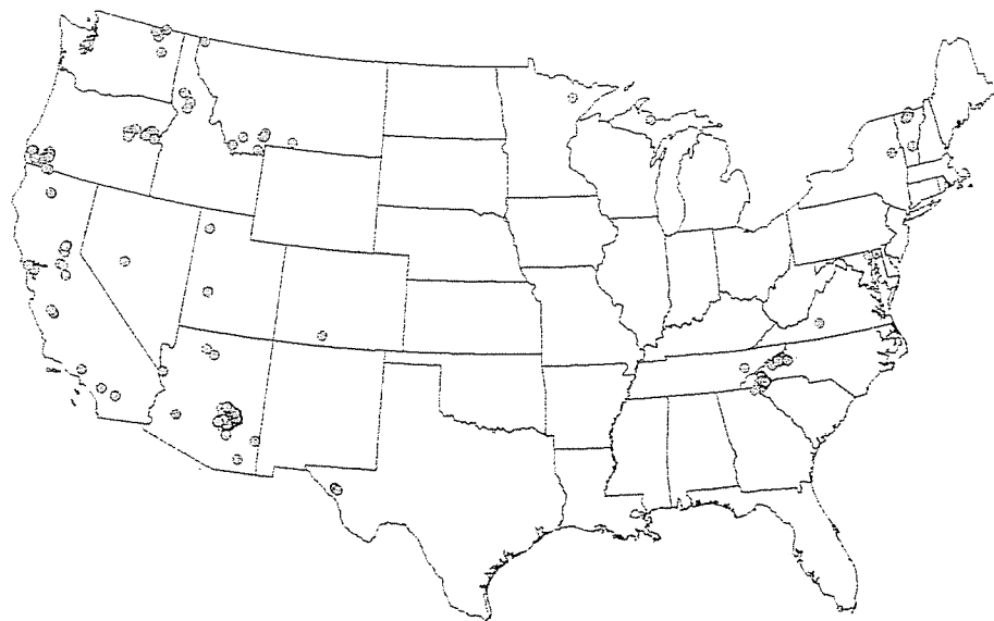
Figure 2. Occurrences of asbestos in the contiguous United States. Major asbestos-bearing deposits occur in the mountain belts in the Eastern and Western United States. Data from USGS Digital Data Series DDS-52 (E.J. McFaul and others, 2000, U.S. Geological Survey Mineral Databases—MRDS and MAS/MILS).
