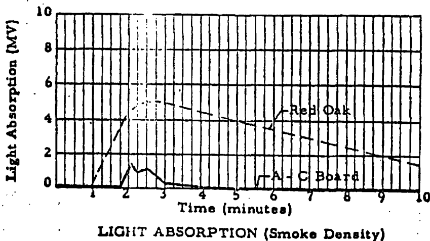
FIGURE 2. GRAPHIC PRESENTATION OF TEST RESULTS FOR SPECIMEN (C)
