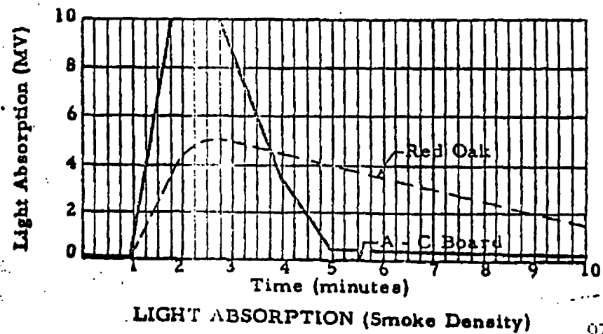
FIGURE 4. GRAPHIC PRESENTATION OF TEST RESULTS FOR SPECIMEN (E)
