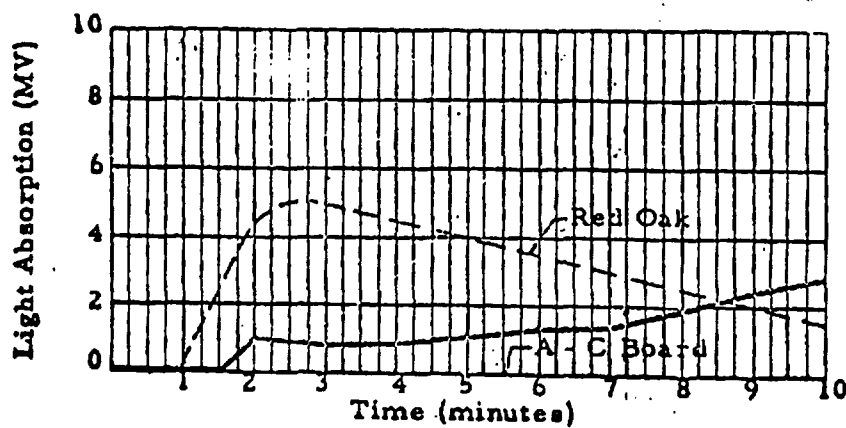
LIGHT ABSORPTION (Smoke Density)
