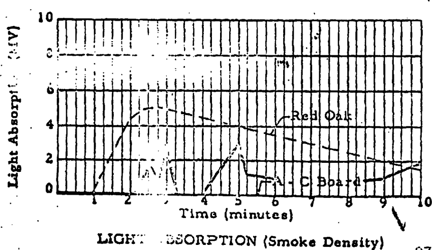
FIGURE 5. GRAPHIC PRESENTATION OF TEST RESULTS
