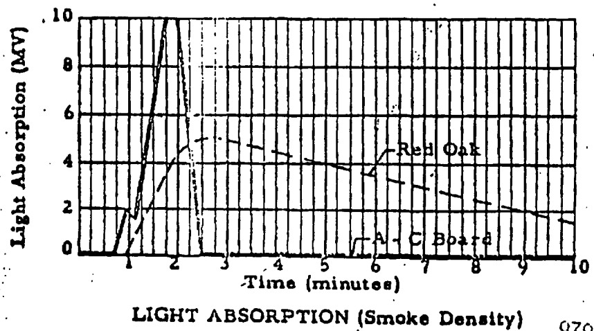
FIGURE 6. GRAPHIC PRESENTATION OF TEST RESULTS FOR SPECIMEN (G)
