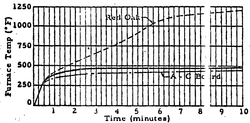
FURNACE TEMPERATURE (Fuel Contribution)
