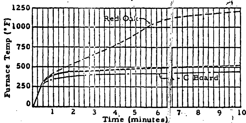
FURNACE TEMPERATURE (Fuel Contribution)
