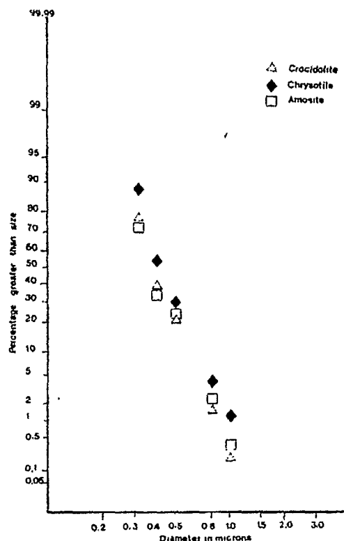
FIG. 2.—Diameter distribution of fibres broader than 0.2 µm. (Scanning electron microscope measurements.)
