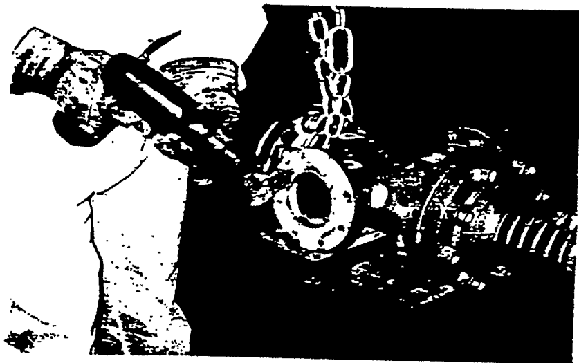
-Photo 6- "Facing" the flange. Fitting #48E is shown.
