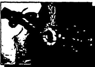
PHOTO 6 - "Facing" the flange. Fitting #48E is shown.
