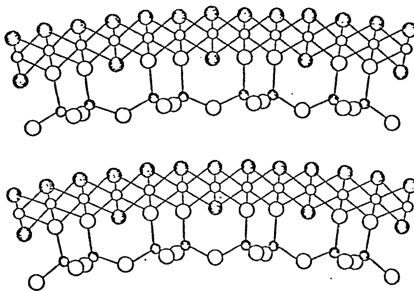
Fig. 2 Simplified chrysotile structure showing the curvature fo crystal planes (after E. Martinez. Can. Inst. Mining & Metallurgy Trans. Vol. LXIX, p. 414-20 1966).
