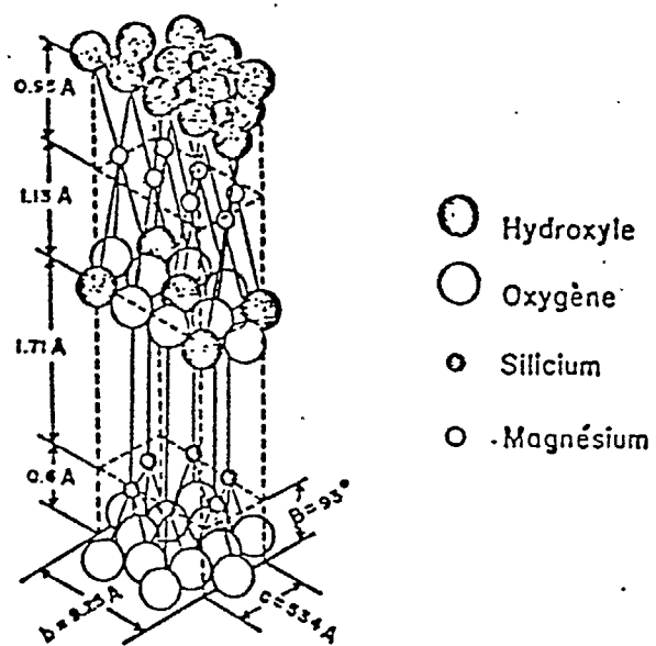
Fig. 1 Unit cell in the crystalline structure of chrysotile (after Cossette, Lemonde and Massey. L'Union Médicale Can 100 759 (1971)).
