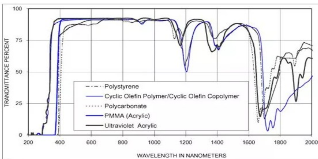
Figure 2. https://www.gsoptics.com/transmission-curves/
