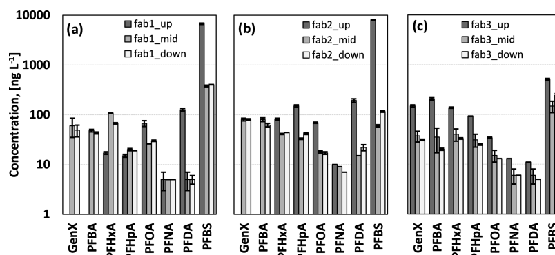
Figure 1. Average concentrations of target PFASs measured in fab wastewater from each of the fabs in upstream samples collected from the photolithography process (dark gray), along the conveyance path as the aqueous wastewater from photolithography is combined with other onsite wastewater (medium gray), and at the point of discharge from the fab (light gray). Note that fab1 and fab3 have onsite biological wastewater treatment plants prior to the point of discharge. Error bars represent the standard deviation of three technical replicates.
