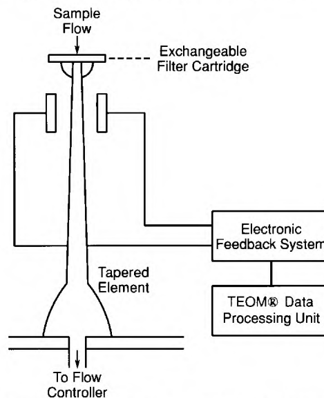
Figure 2.—Schematic of the TEOM® dust sensor.
