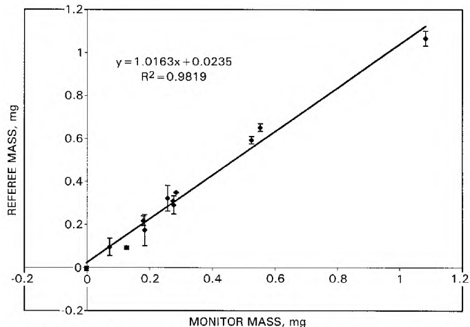
Figure 3.—Mass comparison between referee samplers and the continuous respirable dust monitor.
