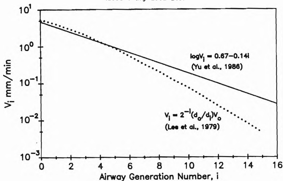
FIGURE 3 Mucociliary Escalator
