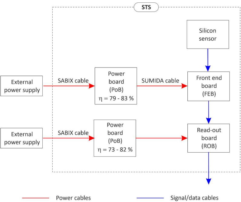
Electronic boards power dissipation per type
