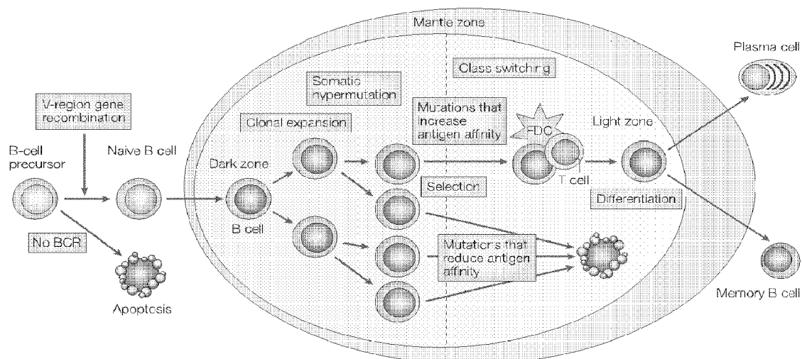
Figure 2 | B-cell differentiation in the germinal-centre reaction. Mature (naïve) antigen-activated B cells that receive signals known as 'T-cell help' are driven into primary B-cell follicles in secondary lymphoid organs such as lymph nodes, where they establish germinal centres (GCs; lightest yellow region) 103 . The naïve IgM + IgD + B cells that constitute the primary B-cell follicle are replaced by the proliferating GC B cells and displaced to the outside of the follicle, where they form a mantle zone around the GC. In the GC, a dark zone and a light zone can be distinguished (left and right sides, respectively). The dark zone mainly consists of proliferating GC B cells, whereas the GC B cells in the light zone are resting 103 . In proliferating GC B cells, the process of somatic hypermutation is activated, which leads to the introduction of mutations at a high rate into the rearranged Ig variable (V)-region genes of the B cells 102 . Most mutations are disadvantageous for the cells—such as those that lead to reduced affinity of the BCR for antigen and cause cells to undergo apoptosis. A few GC B cells will acquire mutations in the BCR that increase their affinity for antigen, and these cells will be positively selected. The selection process presumably takes mainly place in the light zone, where the GC B cells are in close contact with CD4 + T cells and follicular dendritic cells (FDCs). A fraction of these GC B cells undergo class-switch recombination 104 . Finally, GC B cells differentiate into memory B cells or plasma cells and leave the GC microenvironment.
