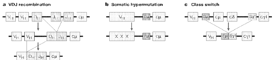
Figure 1 | Molecular processes that remodel immunoglobulin genes. Immunoglobulins (Igs) are expressed by B cells and consist of variable (V) regions, which interact with antigen, and constant (C) regions, which mediate the effector functions of Igs. To create a functional Ig, B cells must rearrange DNA segments that encode the heavy (H)- and light-chain (not shown) regions of the variable genes. a | First, through a process called 'V(D)J recombination', three gene segments, V_H , D_H and J_H , are joined to encode the H-chain variable region. The V regions of the \kappa - and \lambda -light chains, alternatively, are each encoded by two gene segments — the V_L and J_L genes (not shown). B-cell precursors first carry out D_H - J_H rearrangements in H-chain genes. These D_H - J_H rearrangements are followed by V_H - D_H - J_H rearrangements, resulting in the expression of a pre-B-cell receptor if the rearrangement is productive 3 . About 50 functional V_H gene segments, 27 D_H segments and 6 J_H segments are available in the germline, allowing the generation of a diverse repertoire of V_H gene rearrangements. The diversity is further increased by the addition or removal of nucleotides at the joining sites of the gene segments 3 . The cells then carry out rearrangements at their L-chain loci (not shown). The V-region of the Ig gene is ultimately connected to the C-region of the Ig gene ( C_\mu of IgM in diagram) b | The process of somatic hypermutation is activated when B cells reach the germinal centre (GC, shown in more details in FIG. 2). This process leads to the introduction of point mutations, deletions or duplications in the rearranged V-region of Ig genes (denoted by 'X's' in the figure) 192 . These mutations occur in the V-region of Ig genes — not in the downstream C \mu region. c | Class switching results in the replacement of the originally expressed H-chain C-region gene with that of another Ig gene. In the diagram, the C-region for IgM ( C_\mu ) and IgD ( C_\delta ) are exchanged for the C-region of IgG ( C_{\gamma 1} ) by recombination at the switch regions for these genes ( S_\mu and S_{\gamma 1} , respectively). This results in an antibody with different effector functions but the same antigen-binding domain.
