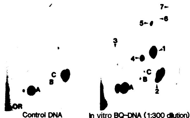
FIGURE 2. Effect of lowering of DNA modifications on the ^{32}\text{P} -postlabeling assay's sensitivity. In vitro BQ-DNA was diluted 300-fold with unadducted kidney DNA and was analyzed by the nuclease \text{P}_1 method. See the legend of Fig. 1 for additional details. Note that chromatographic development in the vertical direction was longer (20 cm) than that performed for maps shown in Fig. 1. Autoradiography was at -80^\circ\text{C} for 15 hr. A, B, and C indicate reference background spots.
