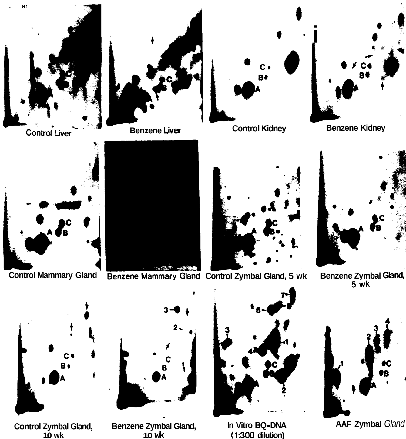
FIGURE 3. Autoradiograms of 32 P-maps obtained with DNA samples isolated from the indicated control and benzene-treated tissues. Autoradiography was performed at -80°C for 48 hr (mammary glands) and 17 hr (others). A, B, and C indicate reference background spots. Adduct 1 seen with AAF-DNA has been identified previously as dpGp-C8-(N 2 -AF) and adduct 2 as dpGp-N 2 -(C8-AAF) (17).
