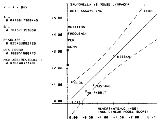
FIGURE 1. Linear regression analysis of the mutagenic activity of diesel and gasoline samples in the S. typhimurium mutagenesis assay versus the L5178Y mouse lymphoma assay. Confidence bands are shown in broken lines.
