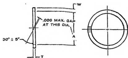
SOLID and SPLIT RINGS—SIZES and DIMENSIONS
