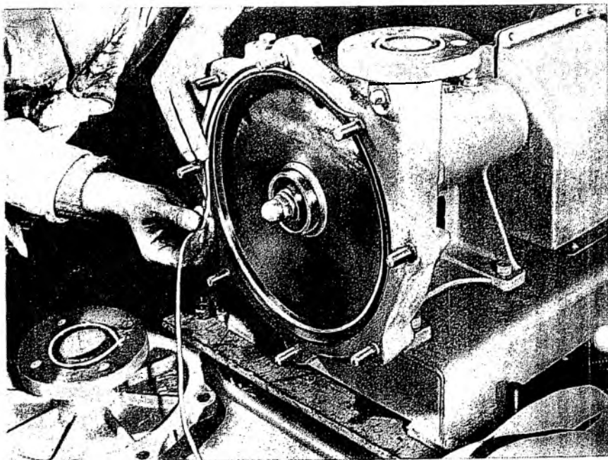
Forming a gasket on a centrifugal pump
