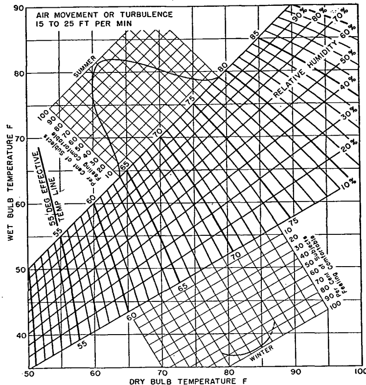
FIG. 10. A.S.H.V.E. COMFORT CHART FOR STILL AIR a,b
