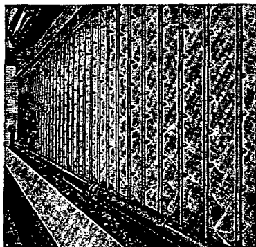
View of Spray Chamber Shaping Nozzles in Operation
