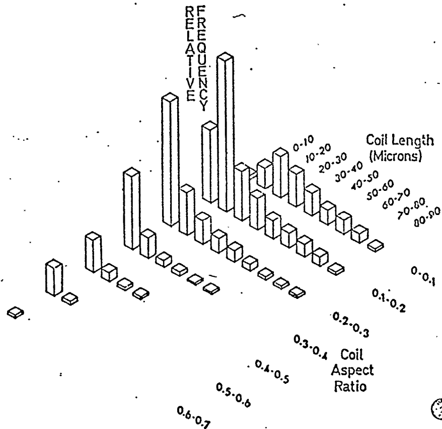
Fig. 3. Distribution of coil length and coil aspect ratio for an industrial chrysotile.
