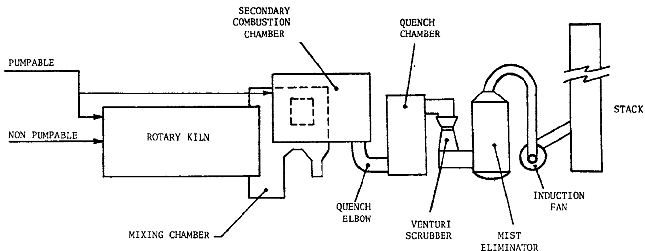
FIGURE 3. Chemolite incinerator schematic.
