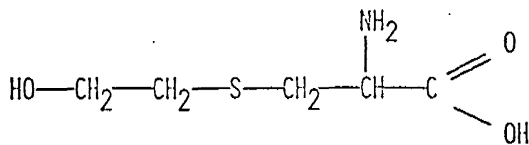
S-(2-HYDROXYETHYL)CYSTEINE
