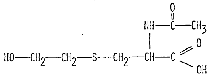
(A) N-ACETYL(S-2-HYDROXYETHYL)CYSTEINE
