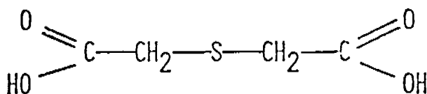
(B) THIODIGLYCOLIC ACID
