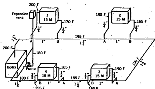
FIG. 13. ONE-PIPE FORCED CIRCULATION SYSTEM
