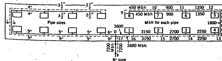
FIG. 15. TWO-PIPE DIRECT RETURN SYSTEM
