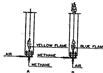
FIG. 3. ILLUSTRATION OF BLUE AND YELLOW FLAME COMBUSTION
