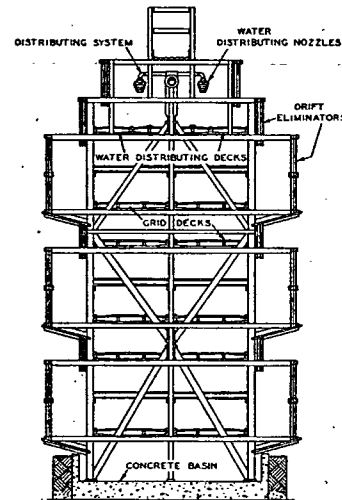
FIG. 6. ATMOSPHERIC DECK TOWER
