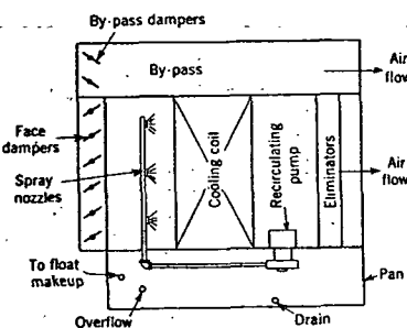
FIG. 11. RECIRCULATING SPRAY SYSTEM FOR CLEANING COILS
