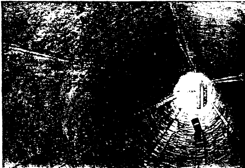
Inside of a lead lined fume duct. Lead strip, as seen in the right foreground, is unrolled to cover the steel straps, which are stud fastened to the vessel shell. The strip is then welded on both sides to protect strap and studs from corrosion.
