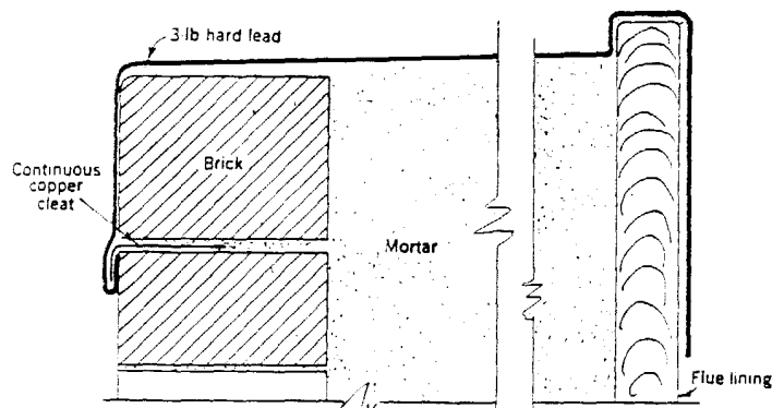
LEAD CAP FOR LARGE CHIMNEY - 2 FLUES - 11' x 4'
