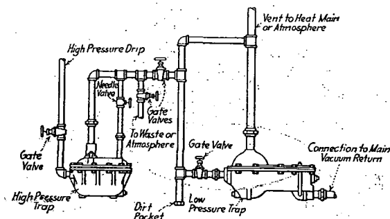
FIG. 20. METHOD OF DISCHARGING HIGH-PRESSURE APPARATUS INTO LOW-PRESSURE HEATING MAINS AND VACUUM RETURN MAINS THROUGH A LOW-PRESSURE TRAP
