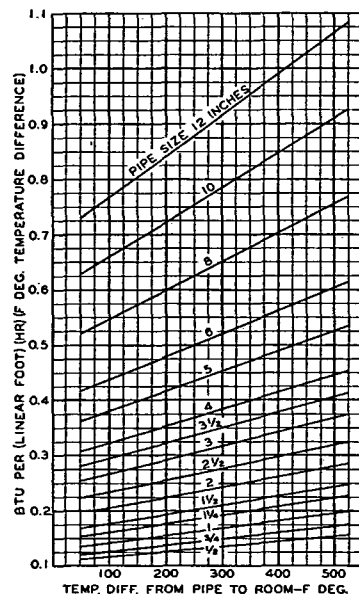
Fig. 2.... Heat Loss through 1 1/2 in. Thick Pipe Insulation (Use with Table 6 for Various Insulations)
