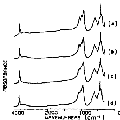
FIG. 1. Infrared spectra of different chrysotile fibers in KBr disk. (a) QS grade 7D, (b) POCl 3 -treated QS grade 7D, (c) QS grade 4T, and (d) POCl 3 -treated QS grade 4T.
