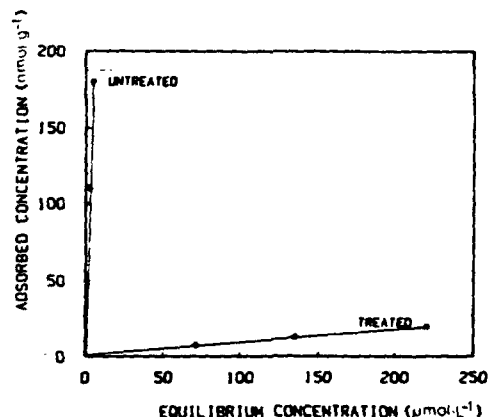
FIG. 3. Adsorption isotherms of benzo[a]pyrene obtained by HPLC technique on the QS 7D fibers.
