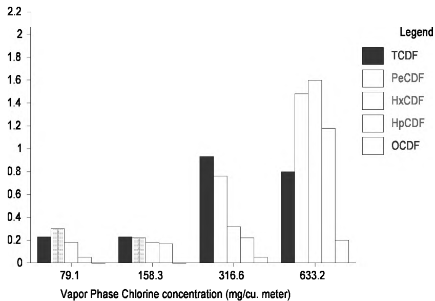
Figure 2-3. The Association Between Vapor Phase \text{Cl}_2 and the Formation of CDDs/CDFs
