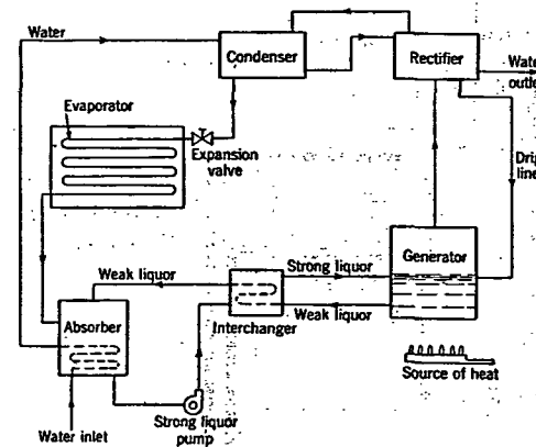
FIG. 7. CLOSED ABSORPTION SYSTEM
