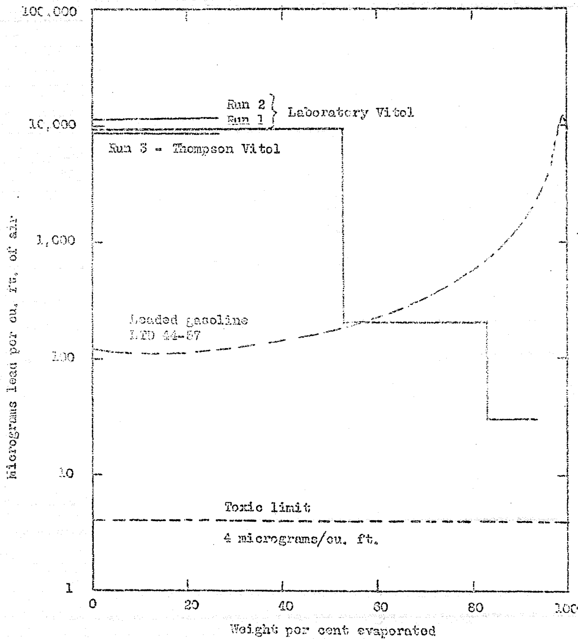
Fig. 3 - Comparison of Lead in Air for Evaporation of Vitol Fluid and Loaded Gasoline.
