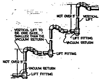
FIG. 16. METHOD OF MAKING LIFTS ON VACUUM SYSTEMS WHEN DISTANCE IS OVER 5 FT
