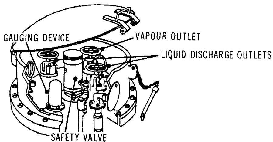
Detail of top unloading arrangement
