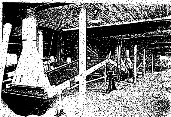
Showing the separating of asbestos fibre from small pieces of rock by suction.
