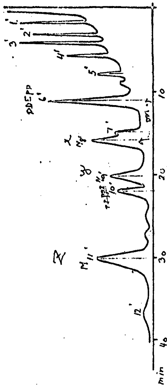
Fig 3. GC-MS chromatogram from eagle sample. Peak numbers represent in points of scanning.
