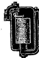
Inverted Bucket Trap
