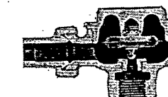
Radiator Trap, No. 1E, 2E, 3C
