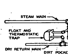
FIG. 41. DRIPPING END OF STEAM MAIN INTO DRY RETURN
