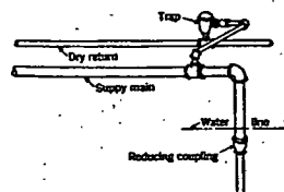
FIG. 40. DRIPPING END OF MAIN INTO WET RETURN
