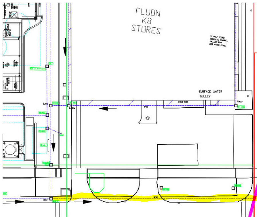
Drainage Plan sheet 5 - Rev B, last updated 03/02/2012
