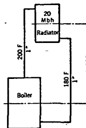
FIG. 7. GRAVITY SYSTEM
