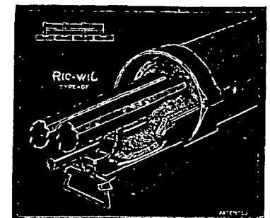
Ric-wiL Type DA is like this DF with insulation moulded to tile but without loose filler.
