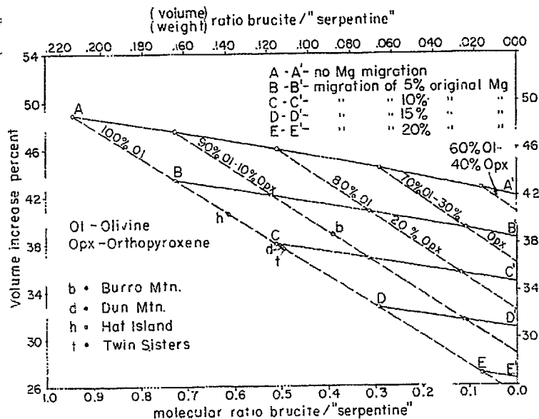
FIG. 2. Volume increase during serpentinization, assuming no addition of silica from surrounding country rocks. Volume increase plotted as a function of original mineralogic composition and resultant brucite/"serpentine" ratios. Molecular amount of migrated magnesium also derived from original mineralogic composition and resultant brucite/"serpentine" ratios. Dun Mountain, Hat Island, Twin Sisters, and Burro Mountain samples shown by solid circles.
