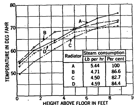
FIG. 6. STEAM CONSUMPTION OF EXPOSED AND CONCEALED RADIATORS
