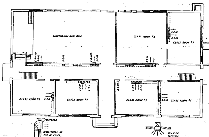
FIG. 8. TYPICAL SCHOOL LAYOUT—FIRST FLOOR PLAN.
