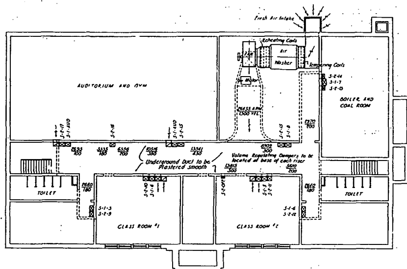
FIG. 7. BASEMENT PLAN CONCRETE DUCT DISTRIBUTION TYPICAL SCHOOL LAYOUT
