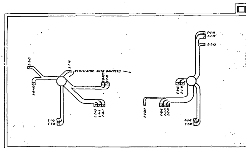
FIG. 10. PLAN OF VENT DUCT IN ATTIC SPACE—TYPICAL SCHOOL LAYOUT
