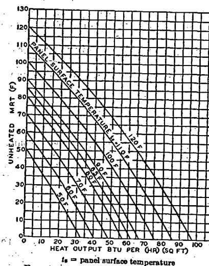
FIG. 9. HEAT OUTPUT BY RADIATION
