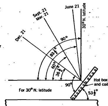
FIG. 11. SOLAR HEATING COIL INCLINATION
