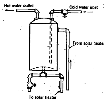
FIG. 10. SOLAR HEATER TANK CONNECTIONS
