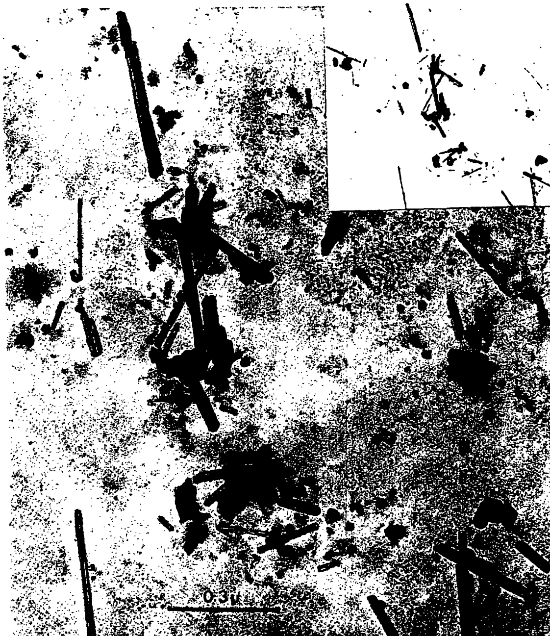
Fig 4.—Chrysotile field at magnification as on EM viewing screen (insert); and photographic enlargement. Even with photographic plate's high contrast, lower-magnification count, only 45 fibers and fibrils were counted; enlargement shows 59 actually present.
