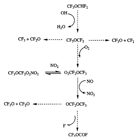
Figure 5. Oxidation mechanism for \text{CF}_3\text{OCHF}_2 (E125).
