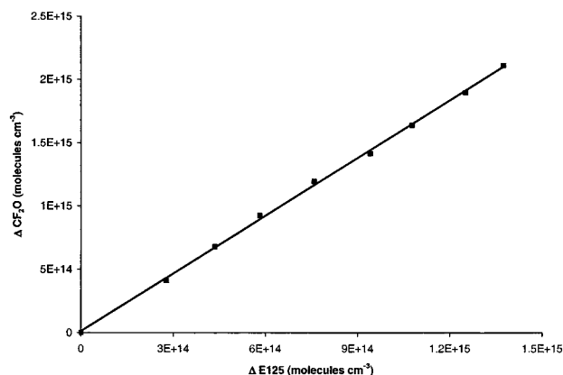
Figure 7. Carbonyl fluoride yield from oxidation of E125.
