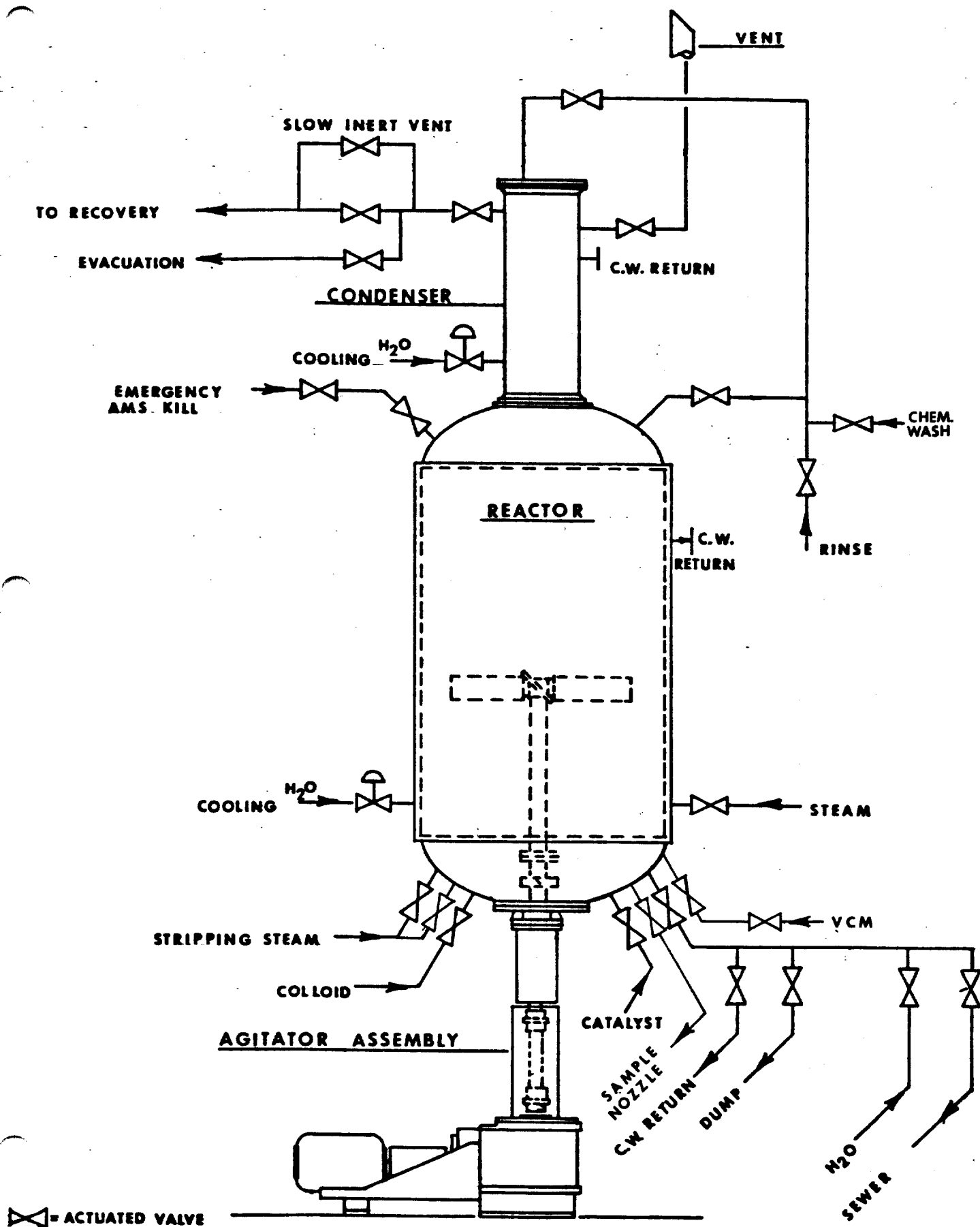
FIG-2 LARGE REACTORS (D-700 & 745)
