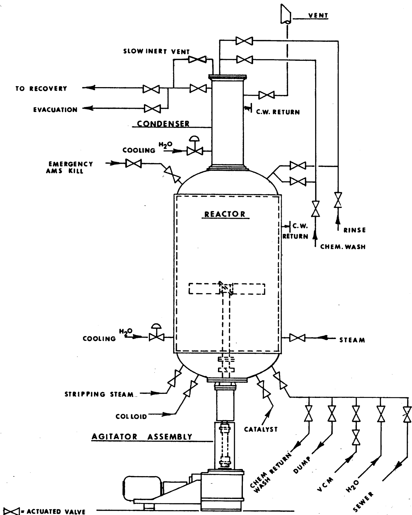
FIG-1 OLD UNIT REACTORS (D-300, 400, 500, 600)
